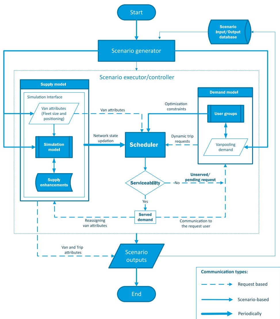
■ Fig. 1. Generic architecture for modeling dynamic vanpooling services
