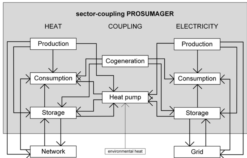
■ Fig. 1. Illustration of possible energy fluxes concerning a prosumer and its system environment
