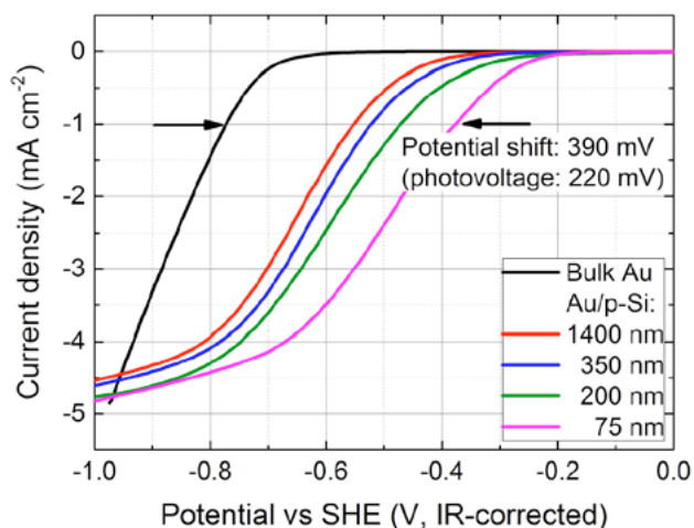
Fig. 1. Linear Sweep Voltammograms of p-Si electrodes covered with different nanostructures of Au or a continuous Au film in buffered KHCO 3 electrolyte saturated with CO 2 under illumination with 444 nm wavelength. A decreasing structure size leads to a drastic reduction of the overpotential (Potential vs. Standard Hydrogen Electrode).
