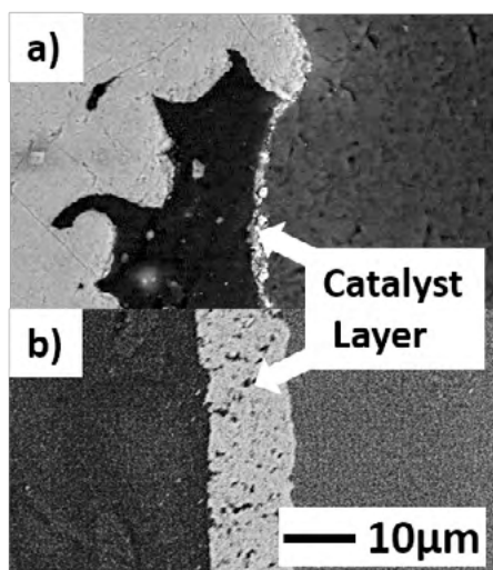
■ Fig. 1. SEM images of iridium-based anode catalyst layers for a PEM electrolyzer at a total loading of ca. 0.2 \text{ mg}_{\text{Ir}}/\text{cm}^2 : a) the conventional catalyst produces an insufficiently thick catalyst layer with poor electronic connectivity and poor activity; b) newly developed catalyst with reduced iridium packing density produces a homogeneous and sufficiently thick catalyst layer with good electronic connectivity and good activity.
